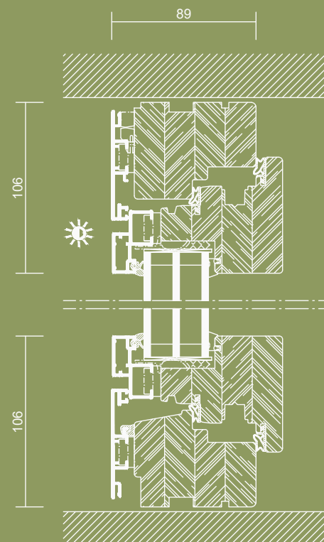
Flush-mounted
