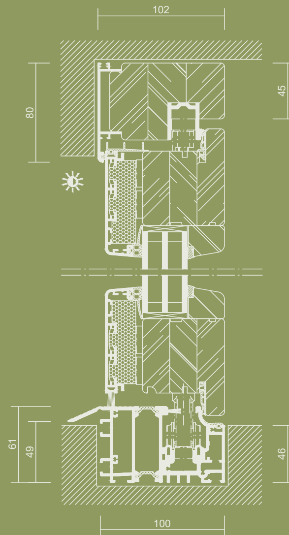
Vertical section | without scale
